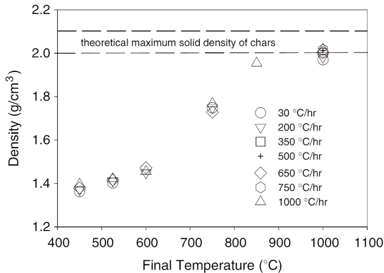
Figure 2.7 Helium-based solid densities of biochars with HTT
