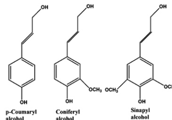
Figure 8.10 Monomers from which lignin is assembled
