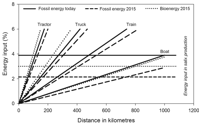
Figure 9.2 Energy use in transportation of wood chips (Salix) as a percentage of energy delivered by the biomass; energy input in Salix production is given as horizontal lines
