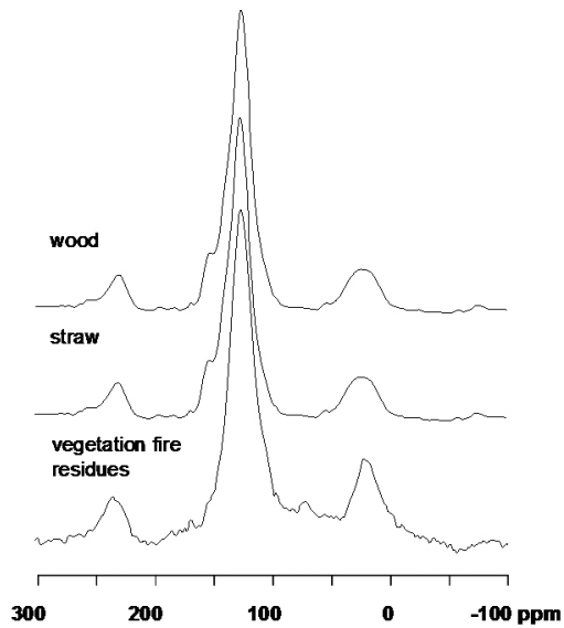
Figure 4.4 Cross-polarization (CP) NMR spectra from biochar derived from wood ( Eucalyptus camaldulensis ) and pea straw ( Pisum sativum ) materials (biochar produced in the laboratory at 450°C in a muffle furnace for 1 hour) and vegetation fire residues from a natural fire
