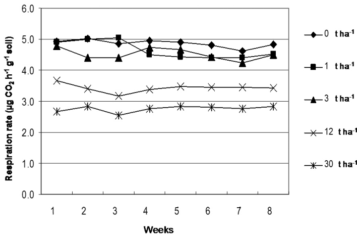
Figure 6.4 Soil respiration rate decreases as the rate of biochar applied increases; incubations of 20g of soil at 50 per cent water holding capacity, CO 2 captured in 0.5M NaOH and quantification of electrical conductivity as a measure of trapped CO 2 (N = 3)
