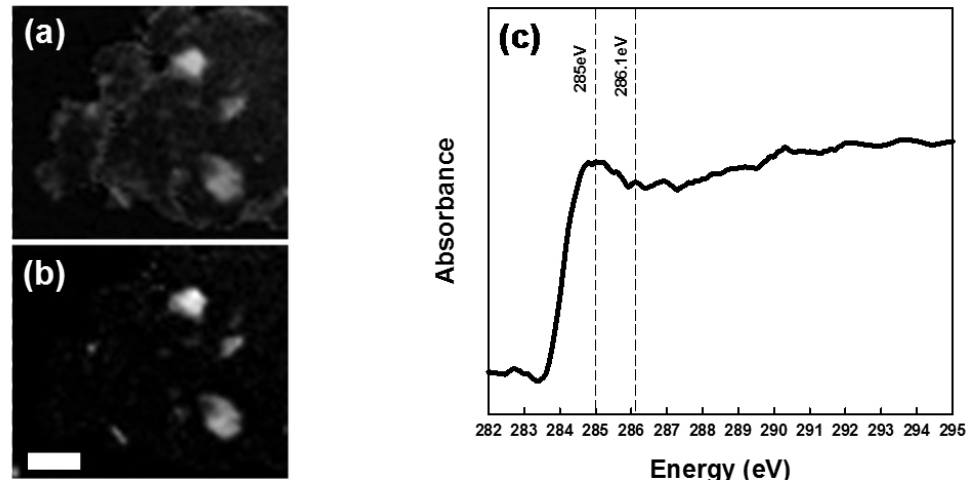
Figure 11.5 Particulate and finely divided biochar embedded within micrometre-size aggregates from a biochar-rich Anthrosol of the central Amazon region. Near-edge X-ray absorption fine structure (NEXAFS) spectroscopy coupled with scanning transmission X-ray microscopy (STXM) of (a) total C and (b) biochar-type C characterized by (c) dominance of aromatic C at 285eV and a characteristic peak at 286.1eV
