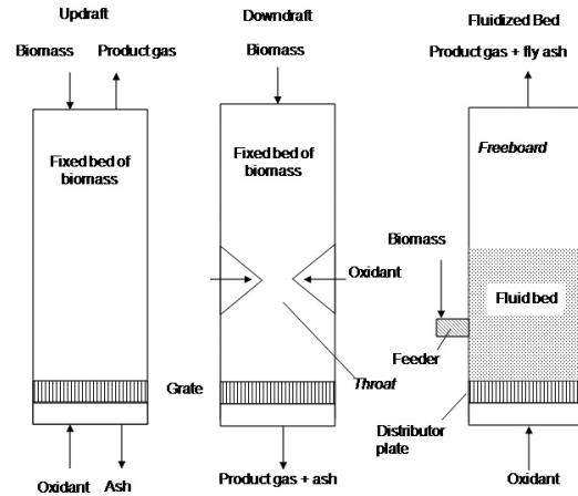
Figure 8.19 Different kinds of gasifiers suitable for co-production of producer gas and biochar
