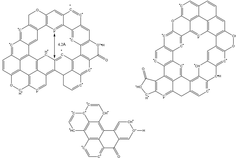
Figure 13.5 Proposed structure of biochar that could interact with N 2 O
