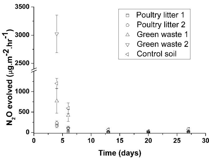
Figure 13.2 N 2 O generated from a Ferrosol amended with biochar in laboratory microcosms
