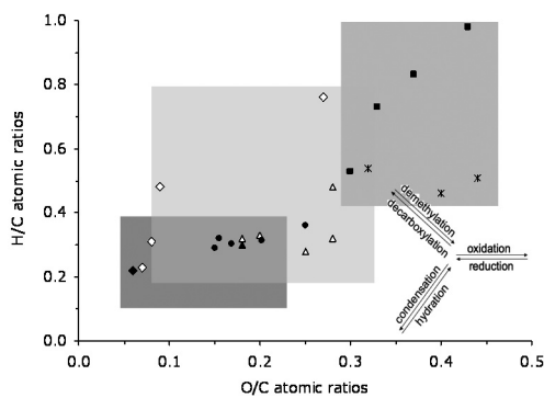
Figure 10.2 Van Krevelen plot of the elemental composition change of (a) furnace hardwood biochar (diamonds); (b) black locust wood biochar (triangles); (c) natural Susuki plant biochar (circles); (d) oven-made Susuki biochar (squares); and (e) red pine biochar with incubation and over time
