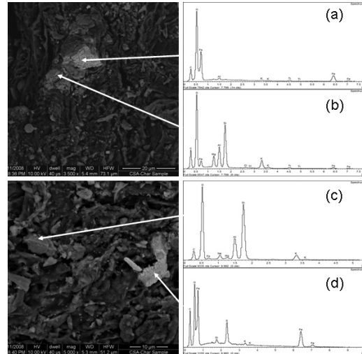
Figure 3.8 SEM micrographs and associated EDS spectra for mineral phases in corn stover biochar prepared by fast pyrolysis: Probable minerals include (a) \text{Fe}_2\text{O}_3 ; (b) dehydroxylated layer silicate or a mixture of \text{Si} , \text{Al} , \text{Mg} and \text{K} oxides; (c) dehydroxylated layer silicate or a mixture of \text{Si} , \text{Al} and \text{K} oxides; and (d) \text{FeS} , \text{FeCO}_3 , \text{S} , \text{Fe}_2\text{O}_3
