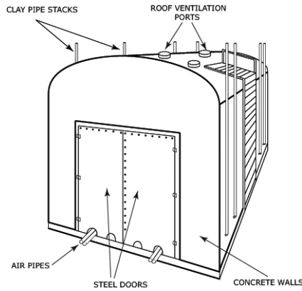
Figure 8.6 The Missouri-type charcoal kiln
