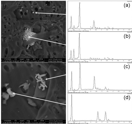
Figure 3.7 SEM micrographs and associated EDS spectra for mineral phases in corn-cob biochar prepared by flash pyrolysis: Probable minerals include (a) \text{Na}_2\text{S} ; (b) \text{Na}_2\text{O} or \text{Na}_2\text{CO}_3 ; (c) \text{ZnS} ; and (d) \text{KCl}
