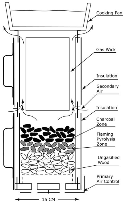
Figure 8.20 Wood-gas stove
