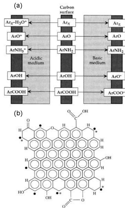
Figure 3.11 (a) Macroscopic representation of the features of C surface chemistry thought to be sufficient for understanding aqueous-phase sorption phenomena; (b) microscopic representation of the functional groups thought to be sufficient for understanding aqueous-phase adsorption phenomena
