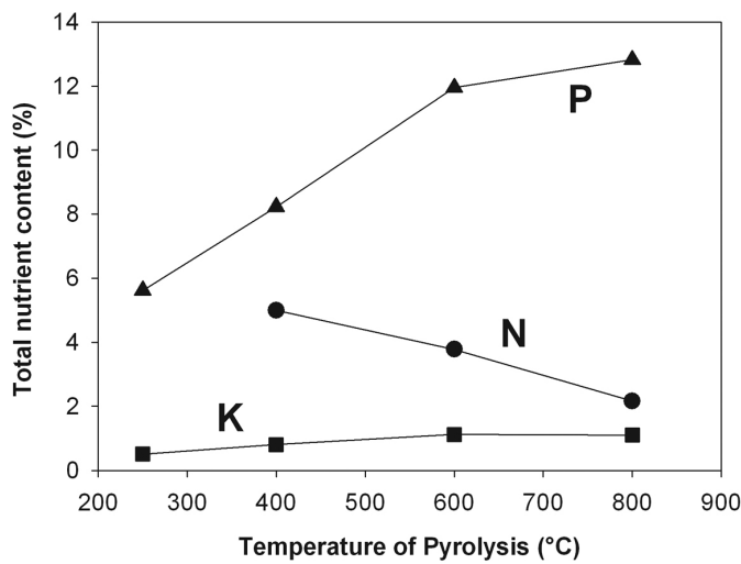
Figure 5.2 Changes in total N, P and K concentrations in biochars produced from sewage sludge at different temperatures
