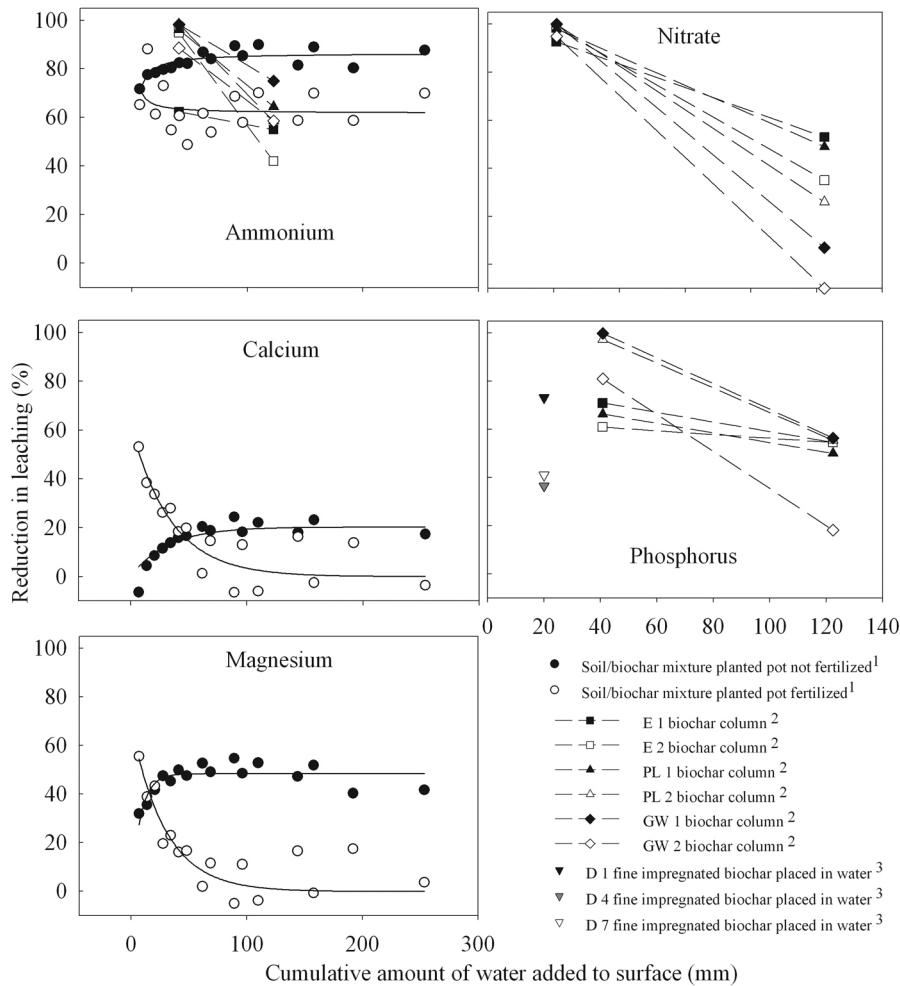
Figure 15.5 Leaching reduction data compiled from the literature: (1) Rice grown in lysimeters filled with Oxisol alone or a mixture of soil and wood biochar, with and without fertilization with NPK (Lehmann et al, 2003); (2) reduction is for NPK fertilizer granules placed on top of columns packed with biochar, compared to a control column packed with acid-washed sand; (E 1) garden waste (GW) biochar made at 550°C, activated, enriched with N; (E 2) GW biochar, same as previous with additional minerals; (PL 1) poultry litter (PL) biochar made at 550°C, activated; (PL 2) PL biochar made at 450°C, non-activated; (GW 1) GW biochar made at 550°C, activated; (GW 2) GW biochar made at 450°C, non-activated (Downie et al, 2007); and (3) reduction is for biochar–ash mixtures compared to original wood feedstock
