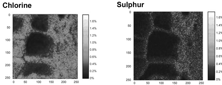
Figure 3.6 Distribution of non-C elements on the surface of wood biochar (produced at 450°C for 0.5hrs) determined by microprobe analysis
