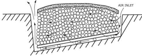
Figure 8.1 Large pit kiln
