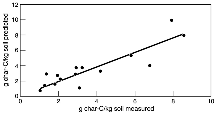
Figure 17.5 Determination of biochar in soil samples, measured using infrared spectroscopy
