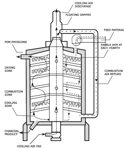
Figure 8.7 The continuous multiple hearth kiln for charcoal production
