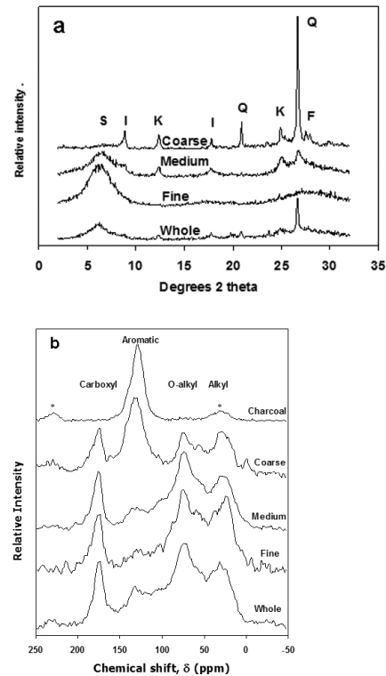
Figure 11.7 Mineralogy (a) and relative proportion of aromatic C (b) forms as an indicator of biochar in coarse (0.2–2 μm), medium (0.02–0.2 μm) and fine (<0.02 μm) clay fractions of a Typic Endoaquoll from Iowa, US
