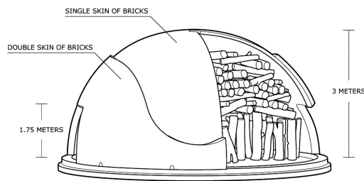
Figure 8.4 Brick kiln
