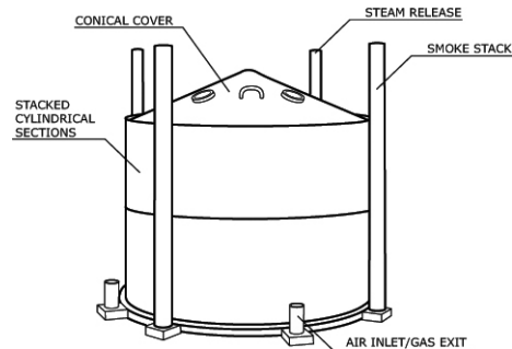
Figure 8.5 Transportable metal kiln, Tropical Products Institute (TPI)
