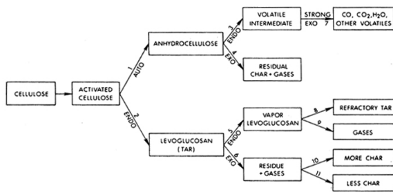
Figure 8.12 Reaction pathways for cellulose decomposition
