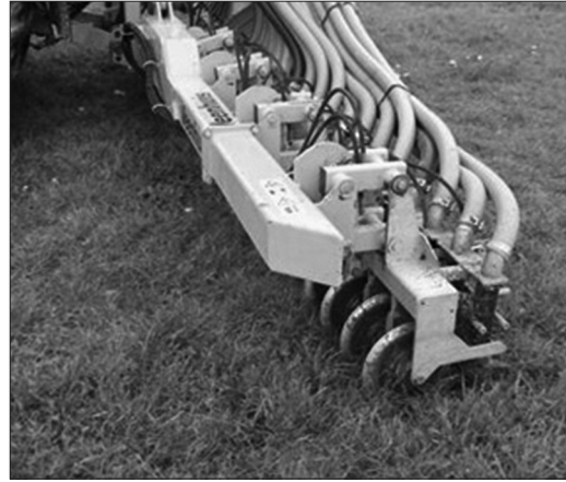
Figure 12.2 Rotary hoeing to mix biochar uniformly in field plots in Bolivia
