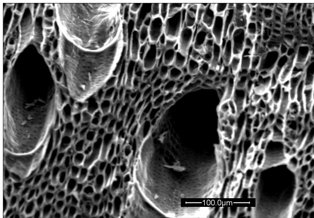
Figure 2.4 Scanning electron microscope (SEM) image showing macro-porosity of a wood-derived biochar produced by 'slow' pyrolysis: The biochar samples were chromium coated and imaged with a beam energy of 20 kV on a FEI Quanta 200 environmental scanning electron microscope (ESEM)
