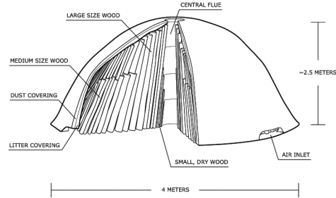
Figure 8.2 Mound kiln
