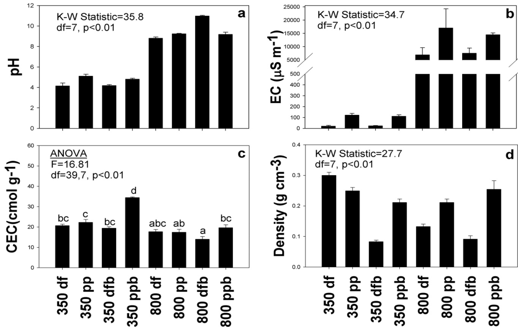
Figure 14.1 The pH, electrical conductivity (EC), cation exchange capacity (CEC) and density of biochar produced from Douglas fir or ponderosa pine wood or bark at 350°C or 800°C
