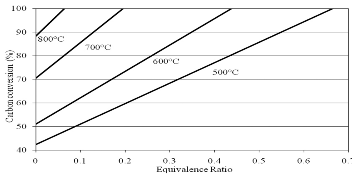
Figure 8.14 Carbon conversion for gasification of cellulose as a function of equivalence ratio (fraction of stoichiometric O requirement for theoretical complete combustion) calculated with STANJAN chemical equilibrium software
