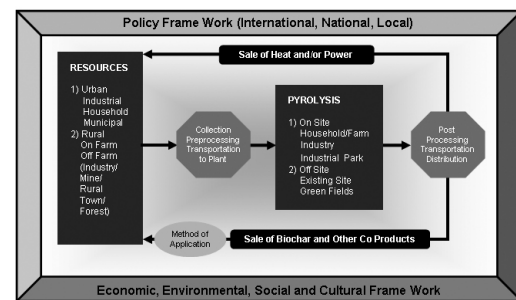
Figure 9.1 Components of biochar systems
