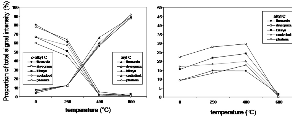
Figure 4.5 Changes in the proportions of O-alkyl, aryl and alkyl C from grass biochars produced at different temperatures
