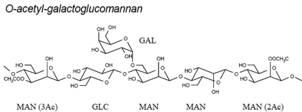
Figure 8.9 Structural formula for a common hemicellulose found in softwoods
