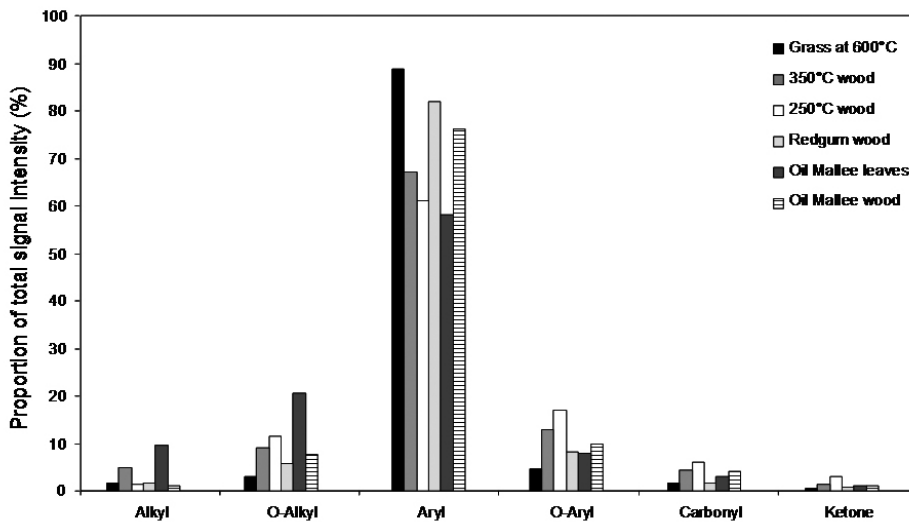
Figure 4.6 Comparison of the proportion of total signal intensity from CP 13 C-NMR of biochars produced at unknown temperatures with those from known temperatures: Data for grass is the average composition of the biochars produced at 600°C from kikuyu, ryegrass, Phalaris and cocksfoot grasses (see Table 4.1); the wood biochars are produced from red pine ( Pinus resinosa )
