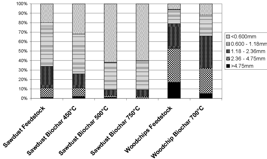
Figure 2.6 Influence of biomass pre-treatment and HTT on the particle size distribution of different biochars
