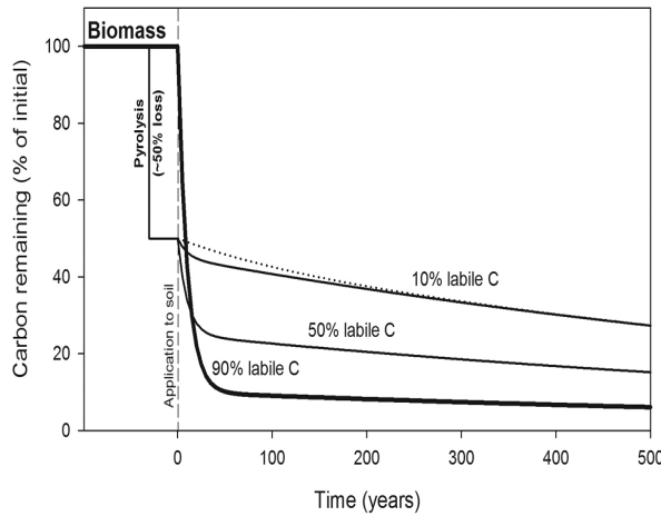
Figure 11.9 Conceptual model of C remaining from biomass using a double-exponential decay model with a mean residence time of 10 years for the labile C pool and 1000 years for the stable C pool, but different proportions of labile C
