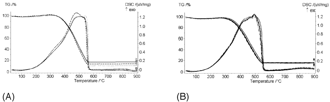
Figure 17.4 Characterization of a reference set of industrial biochars by thermogravimetry and differential scanning calorimetry (TG-DSC) using a Thermal Analyser STA 449C Jupiter (Netzsch type S, Netzsch Instruments, Vigo Place, Aldridge, WS9 8UG, UK) and a PtRh 10 -Pt thermocouple, connected to a Netzsch Aeolus QMS system
